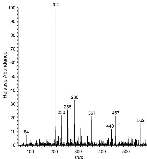
Figure 5. Octapole CID spectrum of [M + 2H]^{2+} ( m/z 562) of pyoverdinin 11 (R = Sucra).
