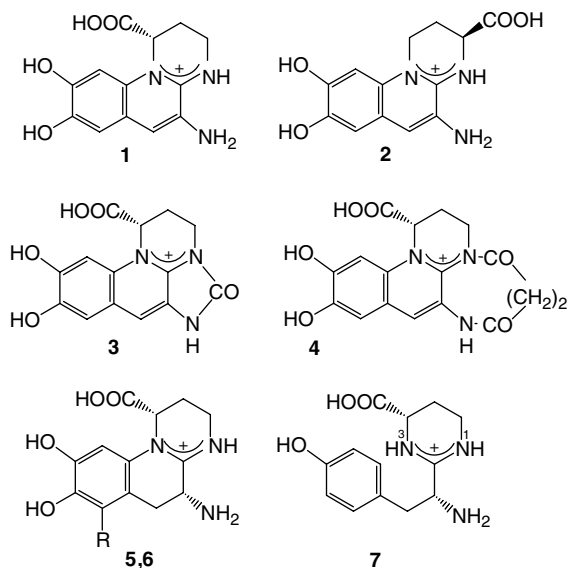
Scheme 1. Chromophores: 1: pyoverdin, 2: isopyoverdin, 3: azotobactin, 4: succinopyoverdin, 5: R = H, dihydropyoverdin, 6: R = SO 3 H, dihydropyoverdin-7-sulfonic acid, 7: ferribactin.
