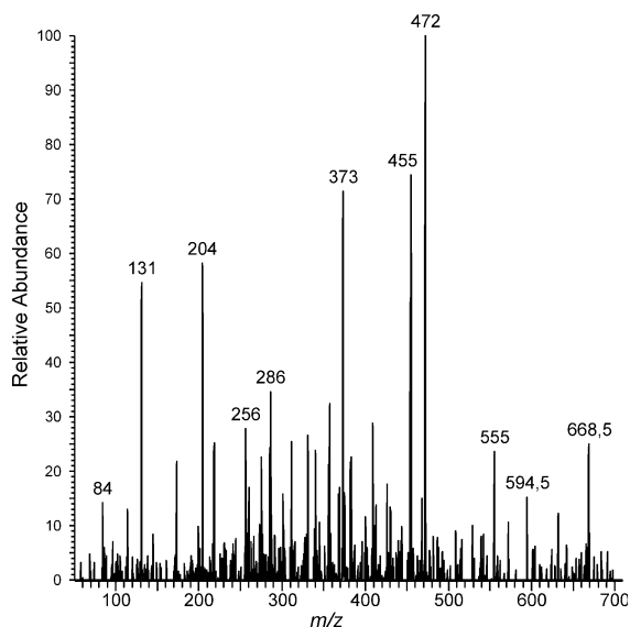
Figure 6. Octapole CID spectrum of [M + 2H]^{2+} ( m/z 668.5) of pyoverdinin 12 (R = Sucra).
