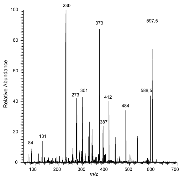
Figure 12. Octapole CID spectrum of [M + 2H]^{2+} ( m/z 597.5) of isopyoverdin 13 (R = Glu).
