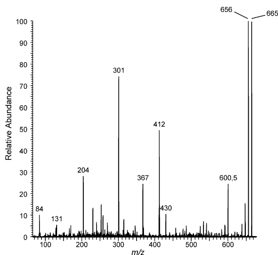
Figure 3. Octapole CID spectrum of [\text{M} + 2\text{H}]^{2+} ( m/z 665) of pyoverdins 9 (R = Glu).
