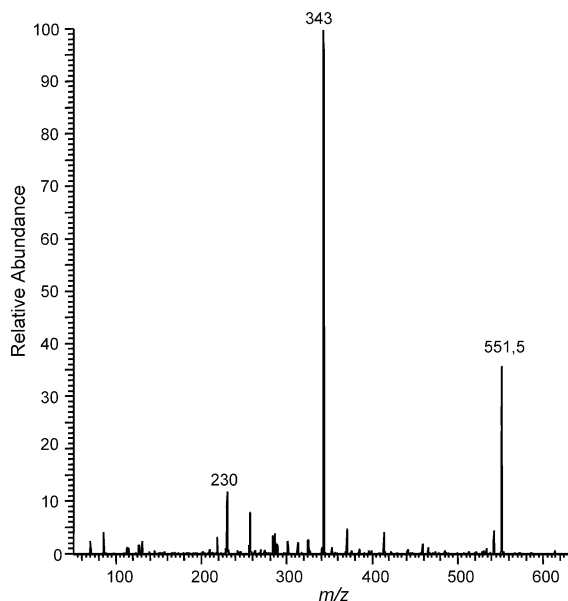
Figure 7. Octapole CID spectrum of [M + 2H]^{2+} ( m/z 551.5) of azotobactin 8 .
