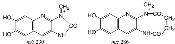
Scheme 6. RDA fragments of azotobactins and succinopyoverdins.
