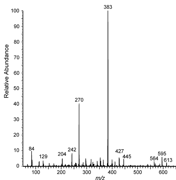
Figure 4. Octapole CID spectrum of [\text{M} + 2\text{H}]^{2+} ( m/z 595) of pyoverdins 10 (R = Kgl).
