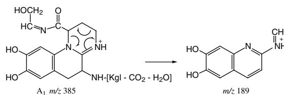
Scheme 7. Characteristic fragment of a dihydropyoverdin.
